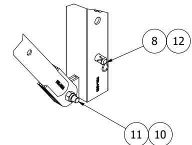
DETAIL D SCALE: 3/32
